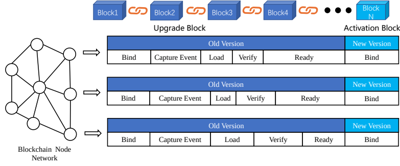
Fig. 2. Node-local preparation and deterministic activation of an EvoCrypt upgrade.
