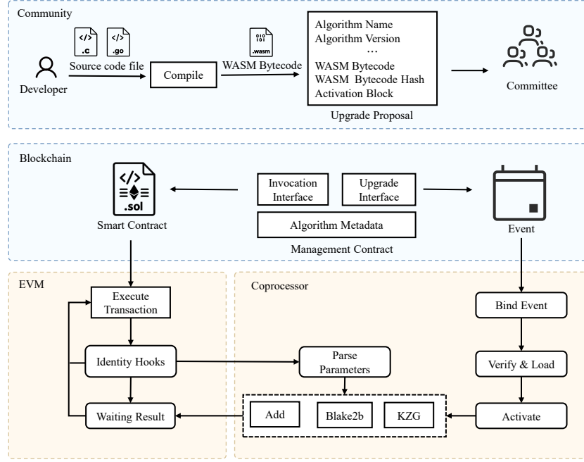
Fig. 1. System model for proposed EvoCrypt framework.
